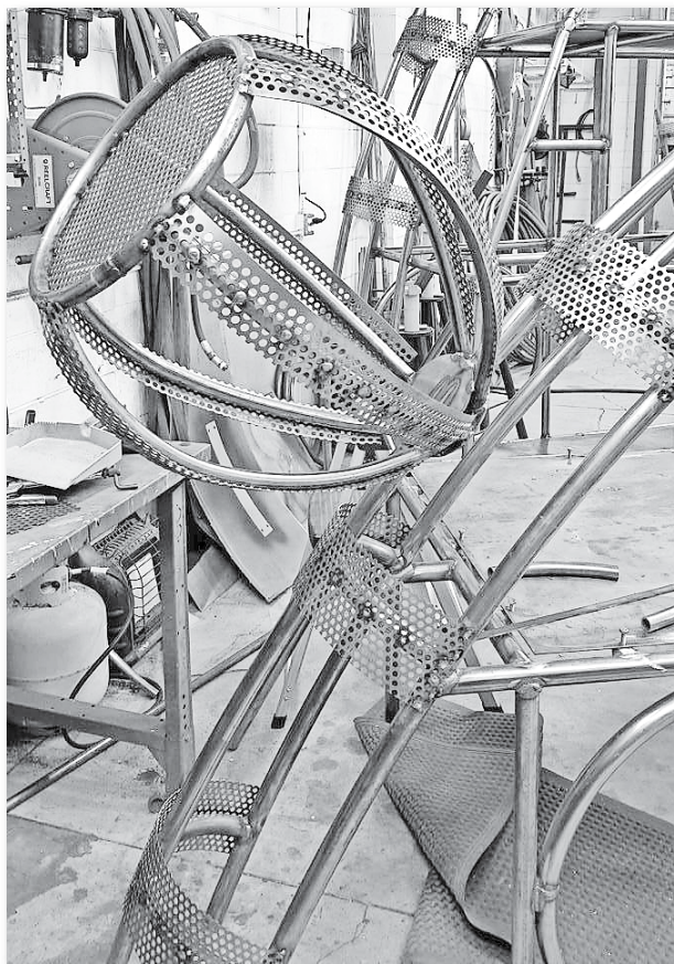
Troy Letwak did the steel work for the Packrat Playhouse and Michael Reddish did the rope work. Michael also designed the project.
